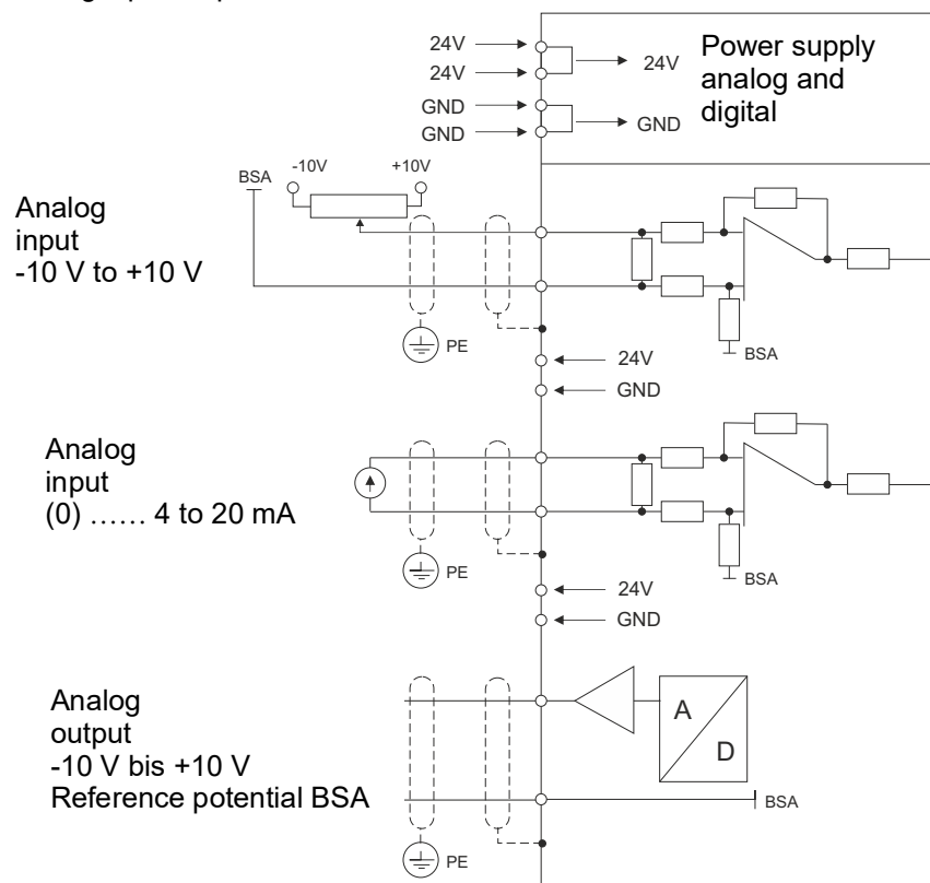
Figure 101: Connection of analog inputs/outputs SVP
