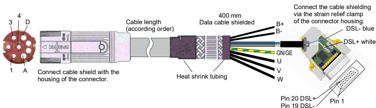
Figure 108: Motor cable with HIPERFACE DSL® 15 A
