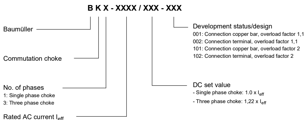
Figure 123: Type code power choke
