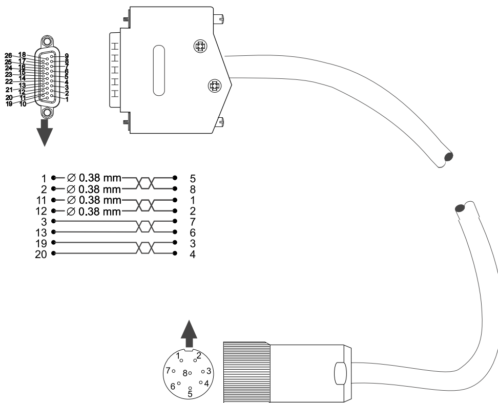
Figure 116: Connecting cable for encoder with EnDat® 2.2 M12
