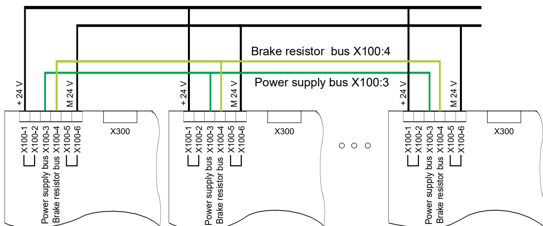
Figure 88: Connection of several devices BM5500 without signal bus
