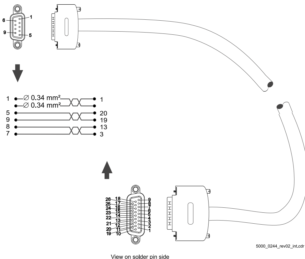
Figure 120: Connection cable SIE with b maXX 5500
