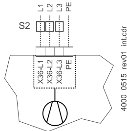
Figure 89: Connection fan BM557X-A
