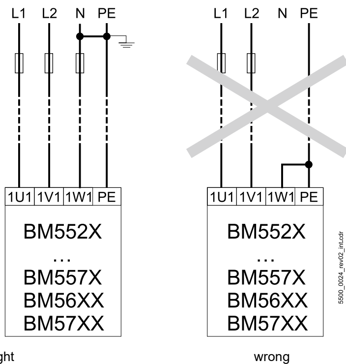
Figure 79: Single phase connection (BM552X ... BM5X7X, basic units)
