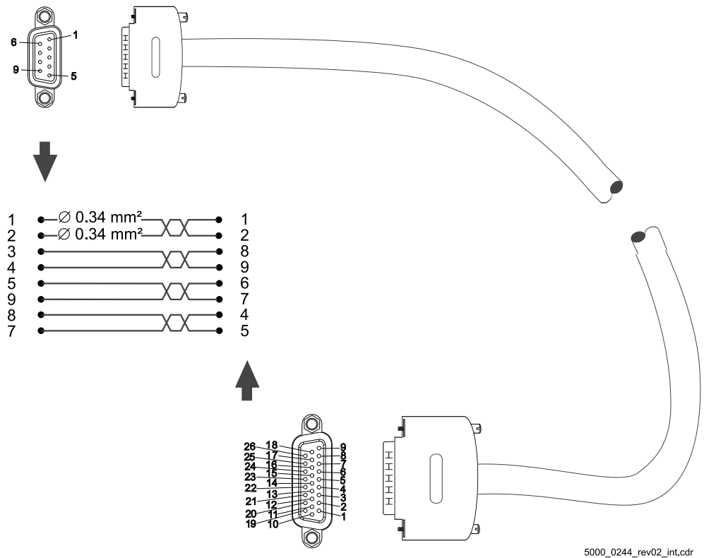
Figure 119: Connection cable IEE with b maXX 5500
