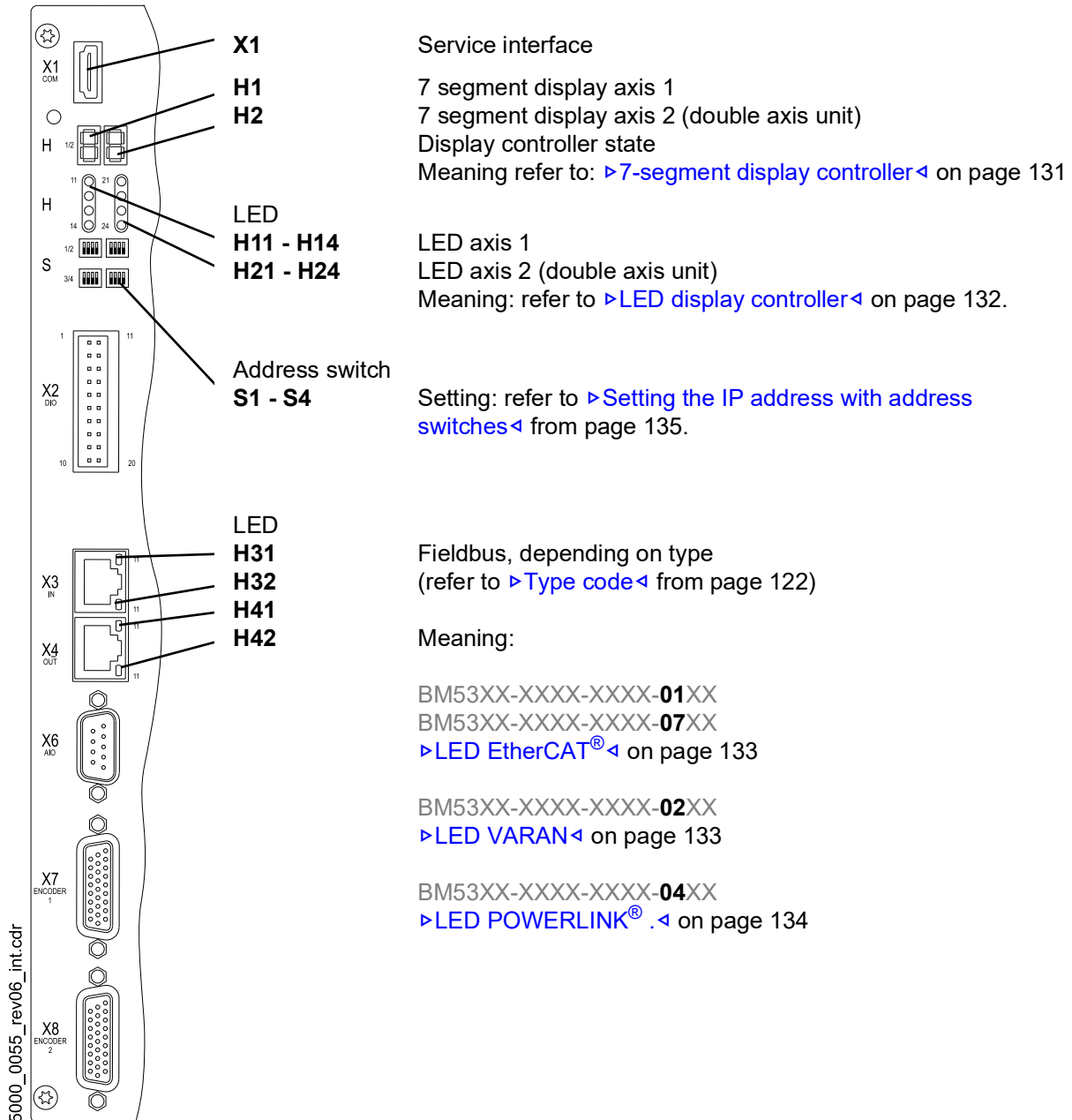
Figure 59: Display/operating elements controller BM52XX, BM53XX
