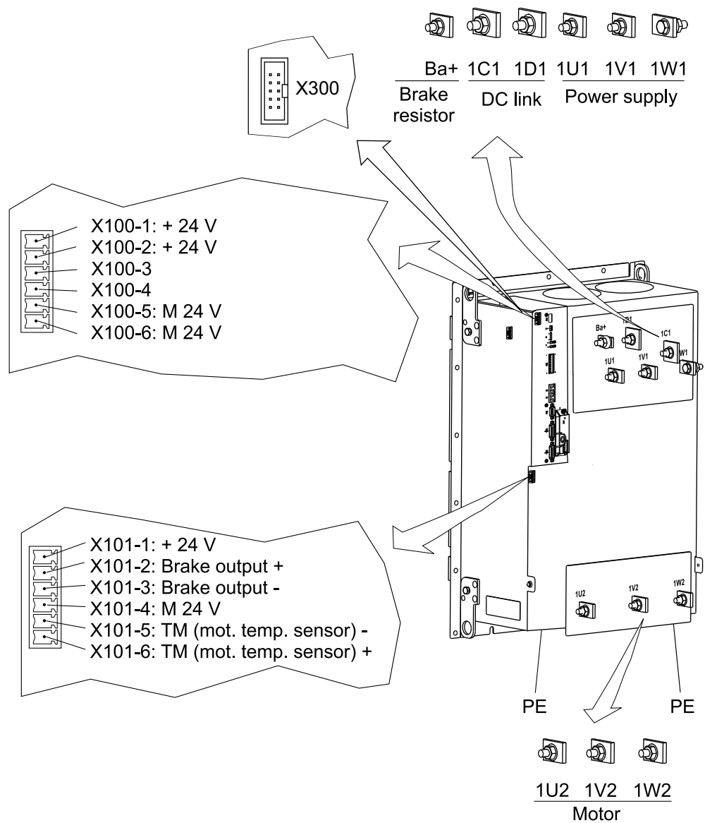
Figure 95: Electrical connections for power supply, motor, ... for BM5X6X
