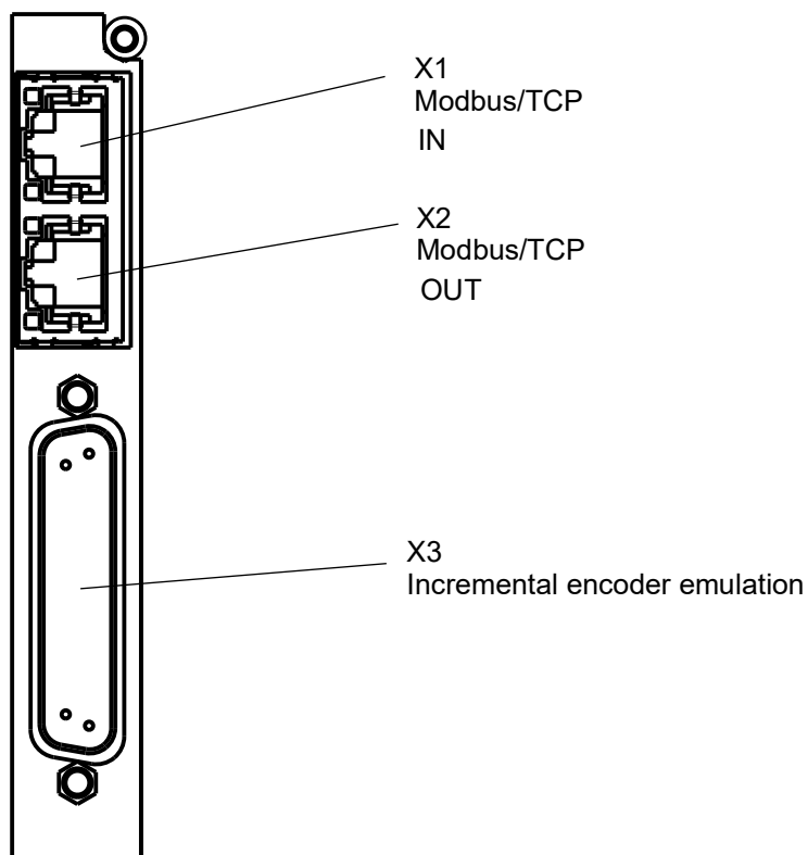
Figure 104: Add-on module Modbus/TCP
