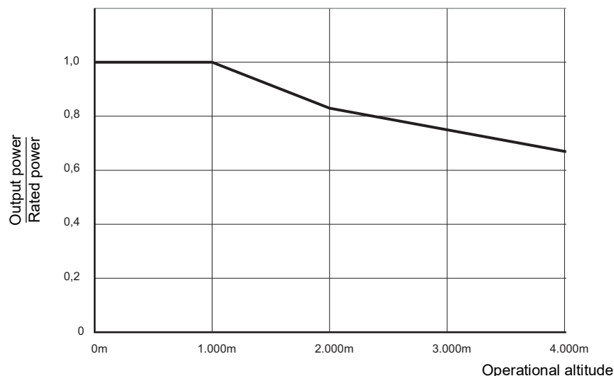
Figure 26: Reducing of the output power in dependence of the absolute altitude
