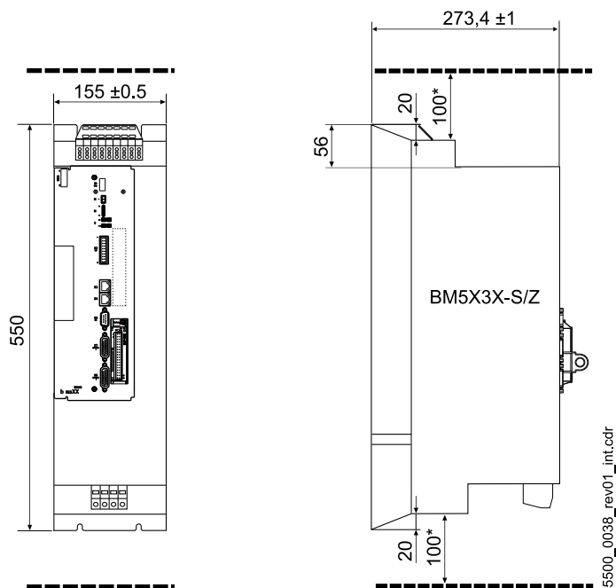
Figure 8: Dimensions BM553X-S/Z
