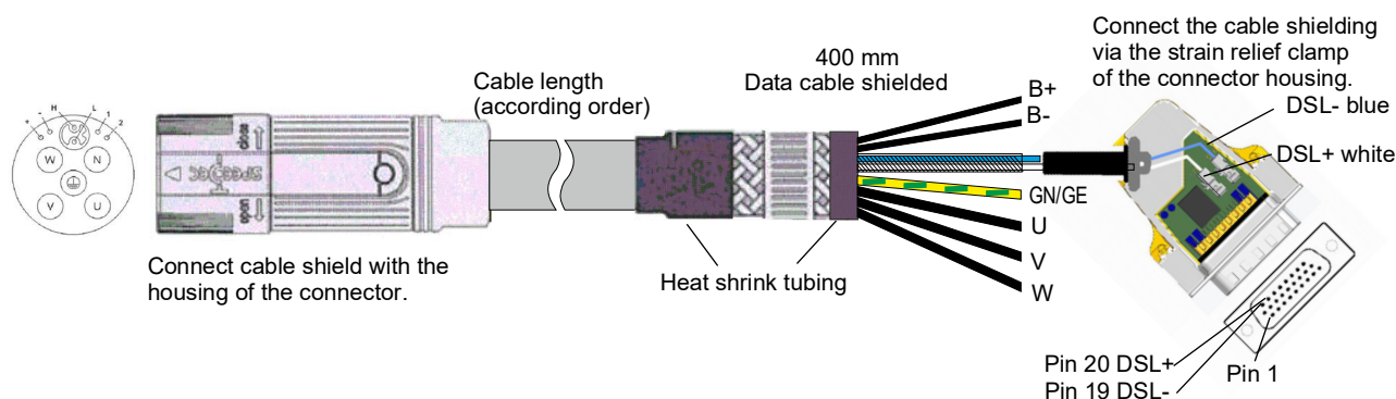
Figure 112: Motor cable with HIPERFACE DSL® 36 A
