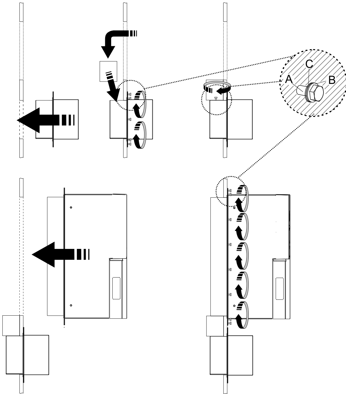
Abbildung 75: Mounting instruction BM557X-A/F, BM577X-FXX9
