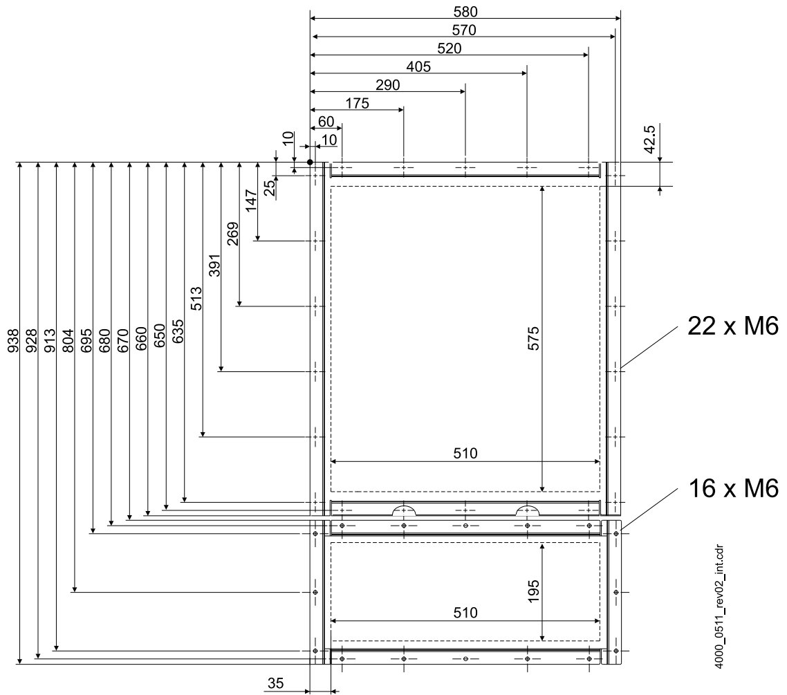
Figure 72: Drilling pattern BM557X-A
