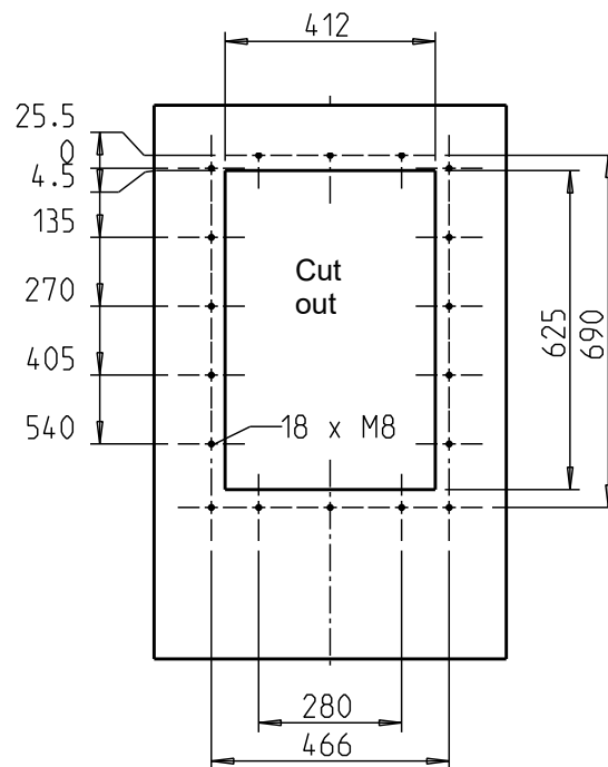
Figure 70: Drilling pattern BM566X-FXX9, BM5766-FXX9
