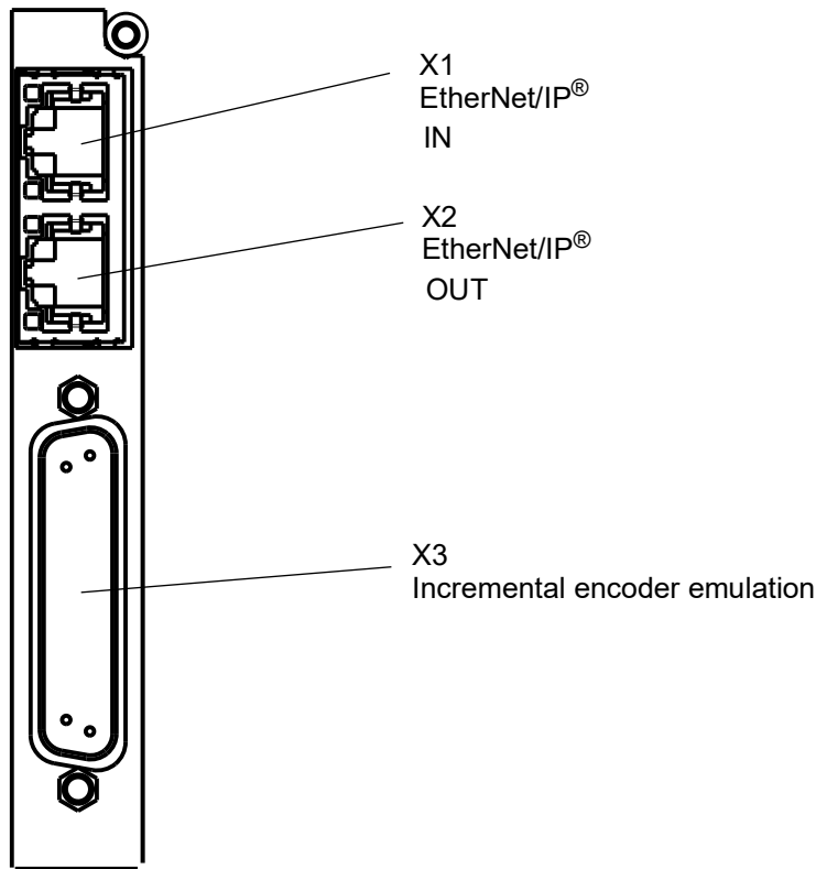
Figure 103: Add-on module EtherNet/IP®
