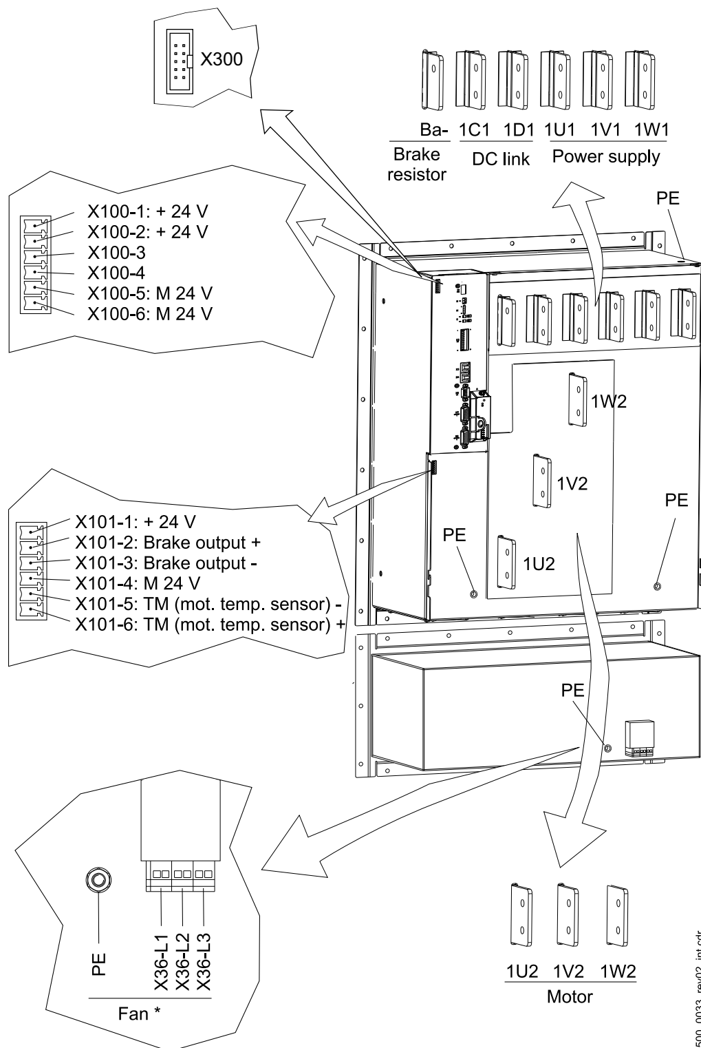
Figure 97: Electrical connections for power supply, motor, ... for BM557X and BM5773
