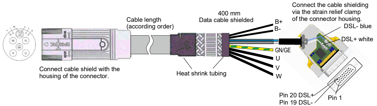
Figure 111: Motor cable with HIPERFACE DSL® 28 A
