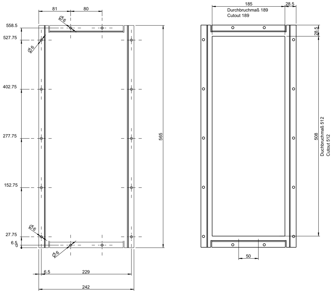
Figure 66: Drilling pattern BM564X-FXX9
