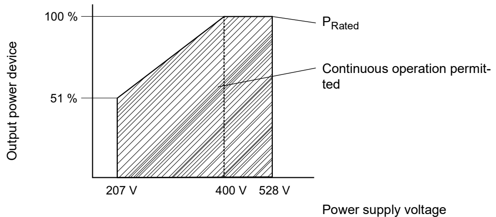
Figure 29: Reducing the output power in dependence of the power supply voltage
