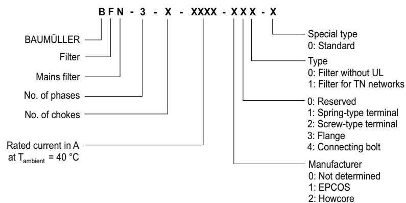
Figure 122: Mains filter type code
