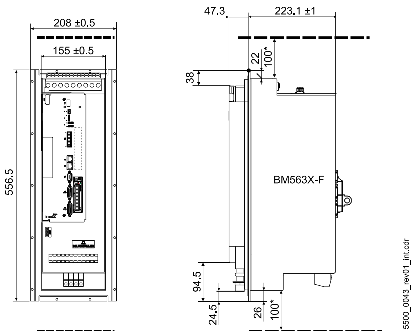
Figure 11: Dimensions BM563X-F
