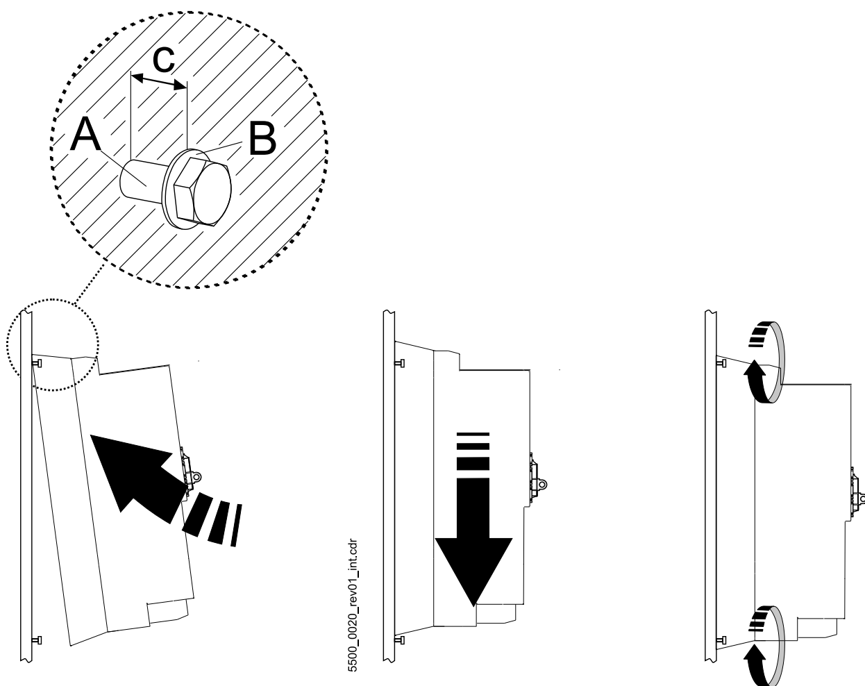
Abbildung 73: Mounting instruction BM554X-S/Z
