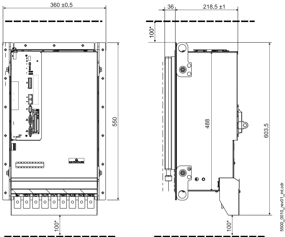
Figure 17: Dimensions BM565X-FXX9, BM575X-FXX9
