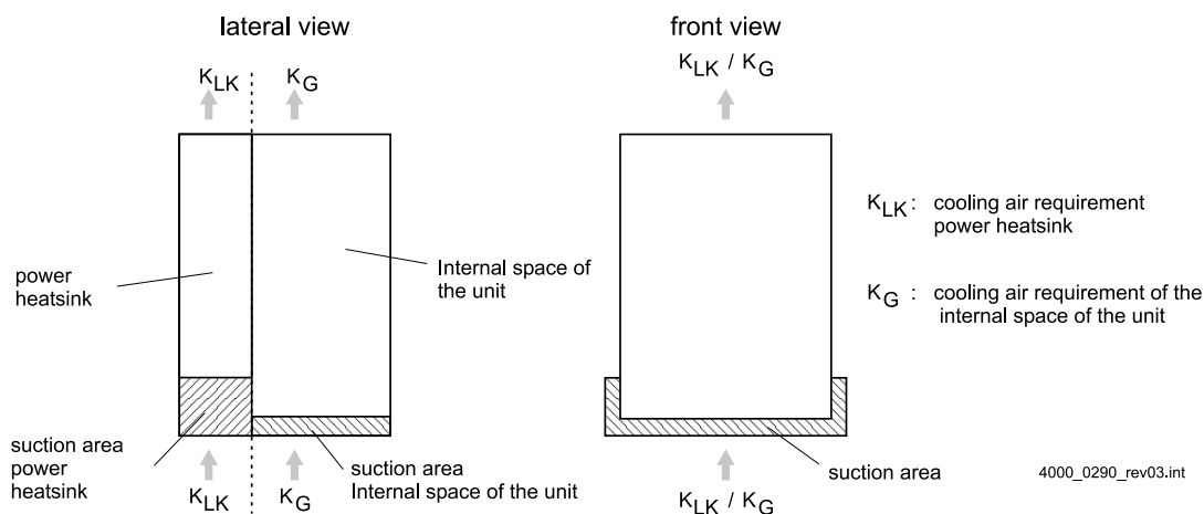
Figure 32: Cooling air requirement
