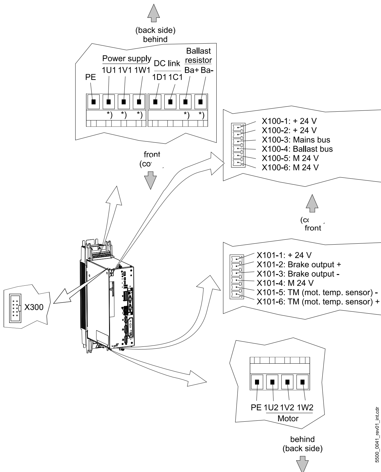
Figure 91: Electrical connections for power supply, motor, ... for BM552X
