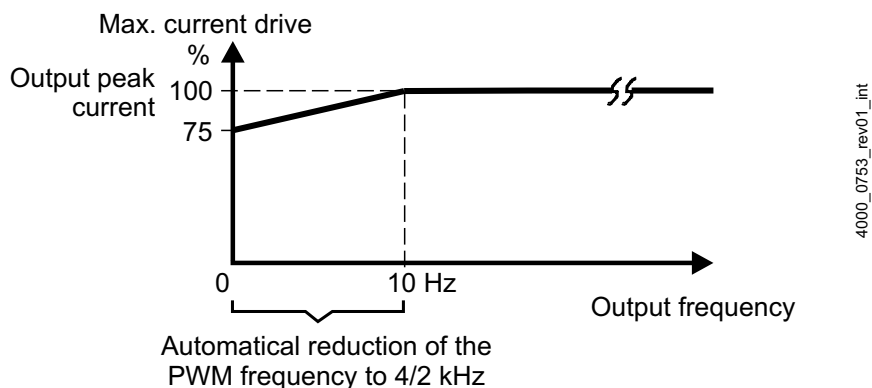
Figure 56: Reduction BM56XX max. current and PWM frequency at output frequencies < 10 Hz
