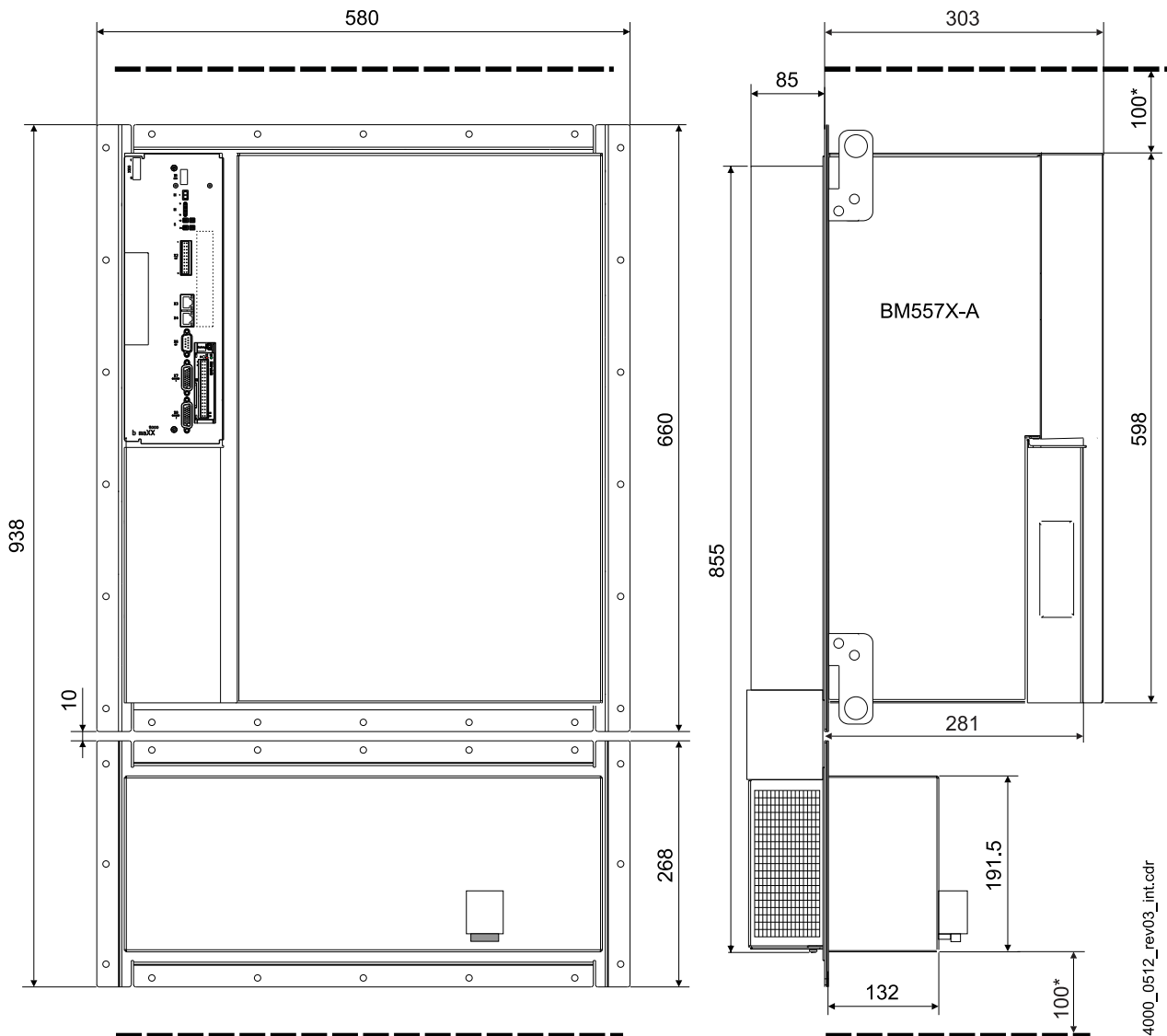
Figure 25: Dimensions BM557X-A
