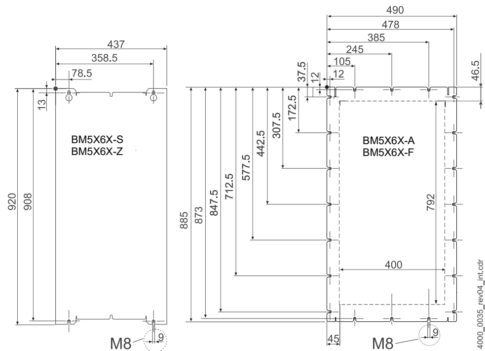
Figure 69: Drilling pattern BM556X, BM565X
