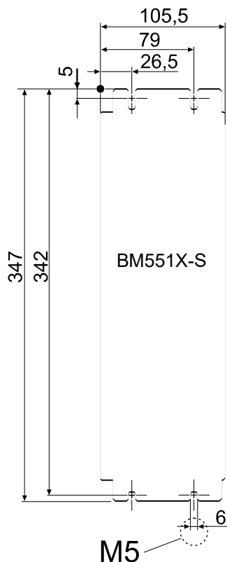
Figure 62: Drilling pattern BM551X
