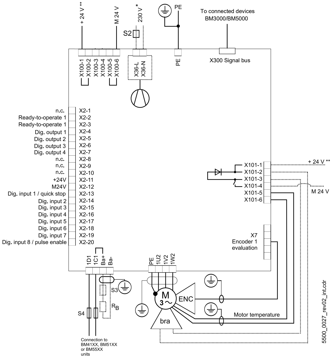
Abbildung 85: Connection diagram with a directly controlled motor brake - power modules
