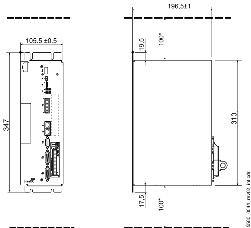
Figure 5: Dimensions BM551X
