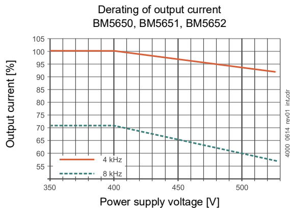
Abbildung 44: Derating the output current BM565X acceleration units
