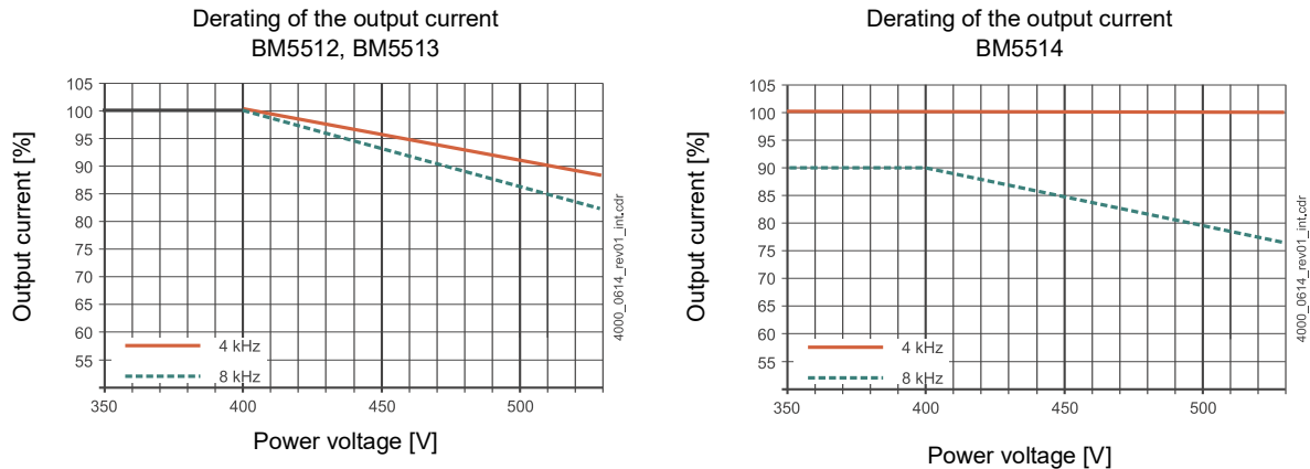
Figure 33: Derating the output current BM551X universal units
