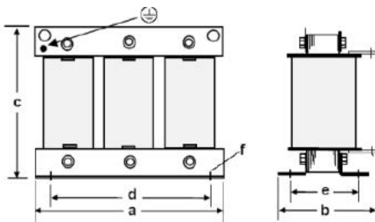
Figure 124: Figure power choke
