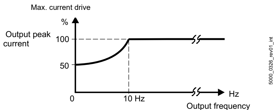
Figure 57: Reduction BM56XX only max. current at output frequencies < 10 Hz
