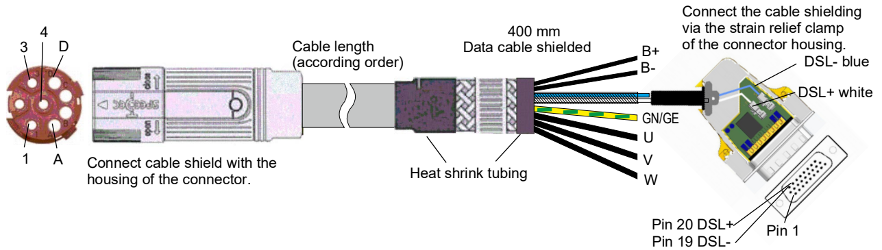
Figure 109: Motor cable with HIPERFACE DSL® 20 A
