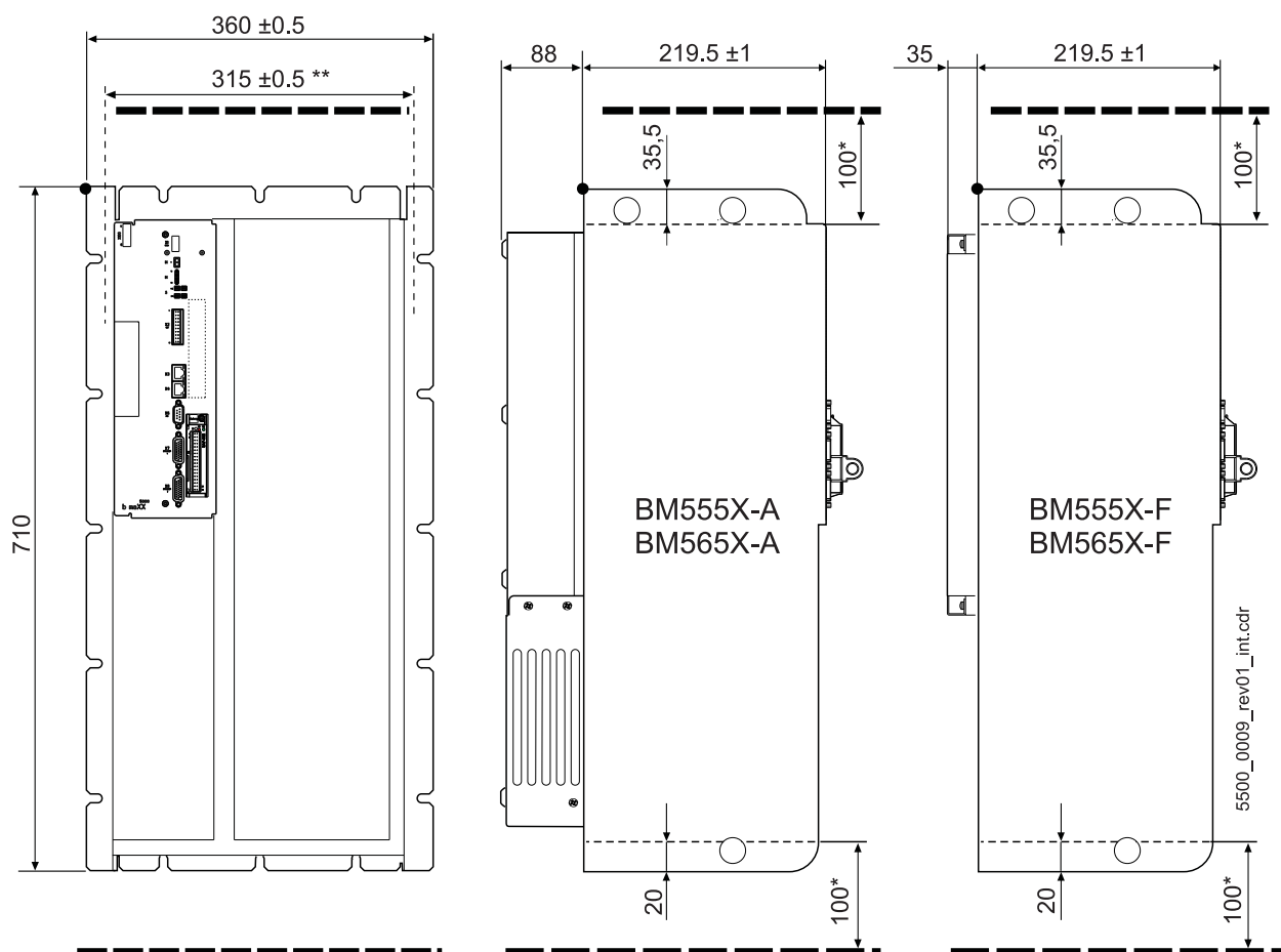
Figure 16: Dimensions BM555X-A/F
