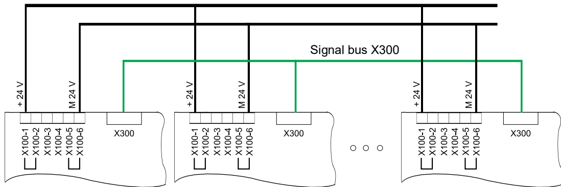
Figure 87: Connection of several devices BM5500 via signal bus
