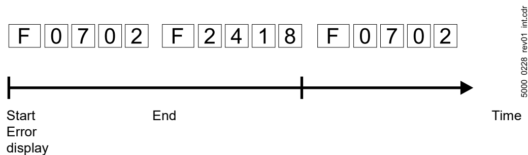
Figure 107: 7-segment display : errors and warnings
