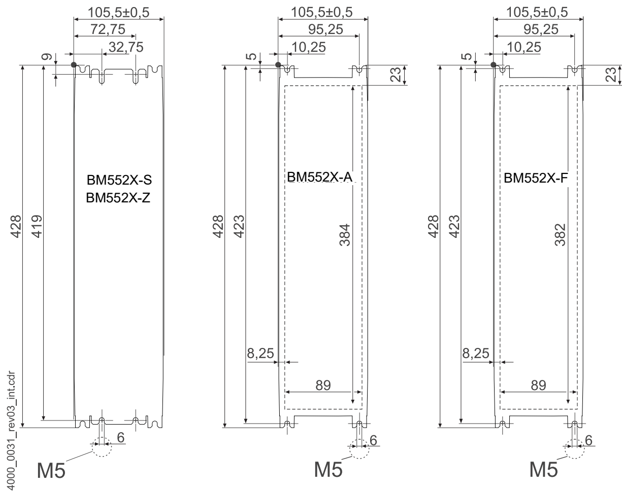
Figure 63: Drilling pattern BM552X
