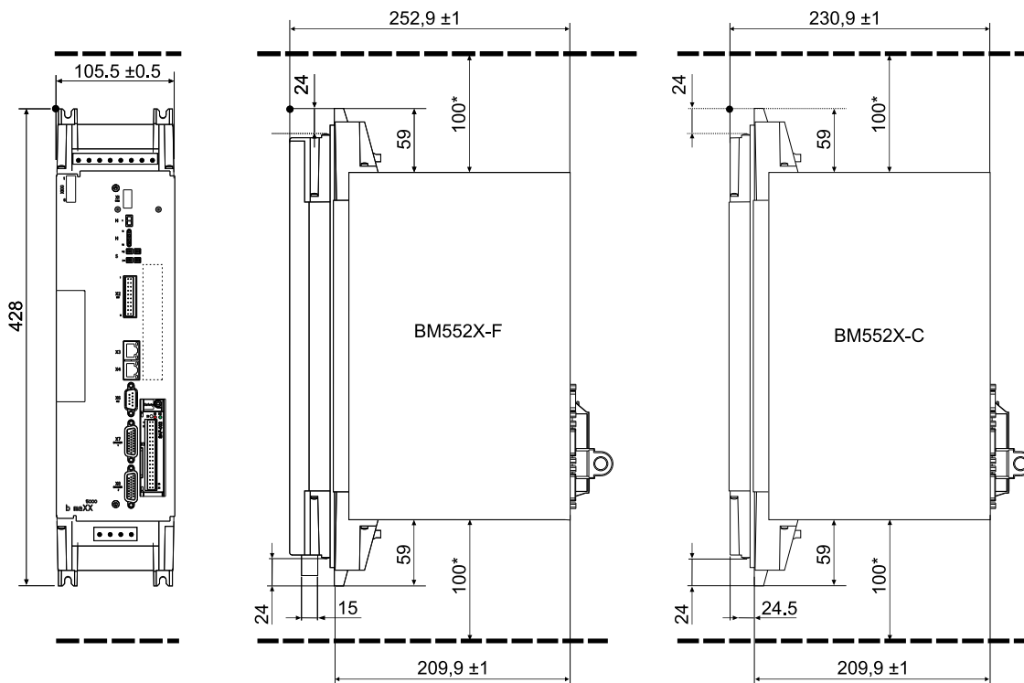
Figure 7: Dimensions BM552X-F/C
