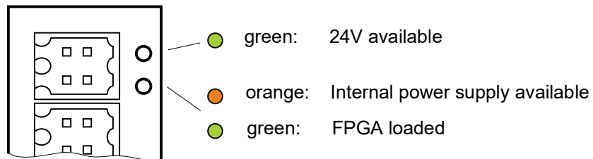
Figure 100: LED display add-on module SVP
