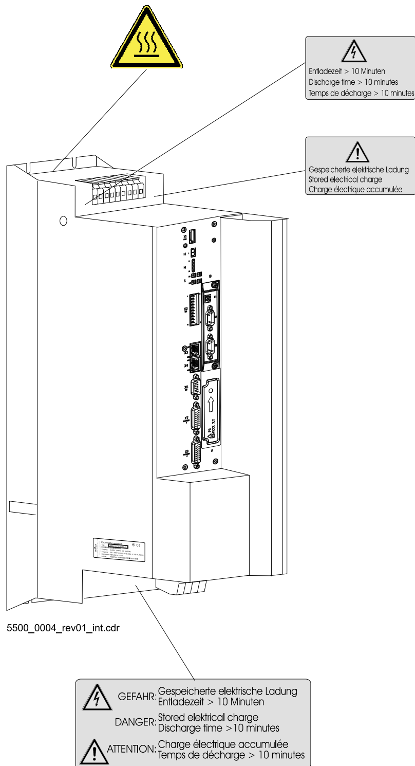
Abbildung 3: Signs and labels BM5X4X, BM5X5X
