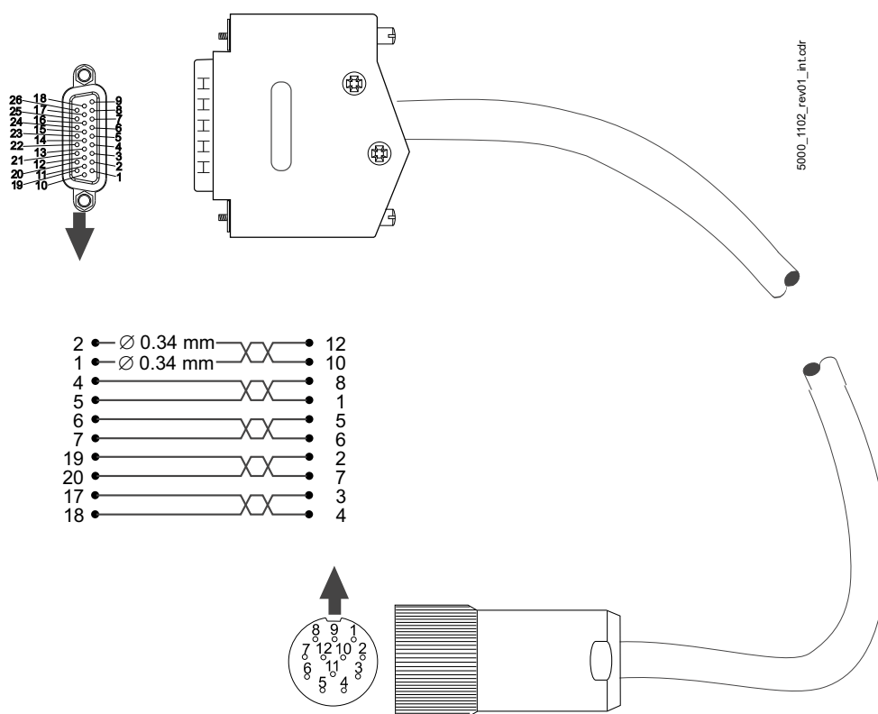
Figure 114: Connecting cable for encoder with HIPERFACE®
