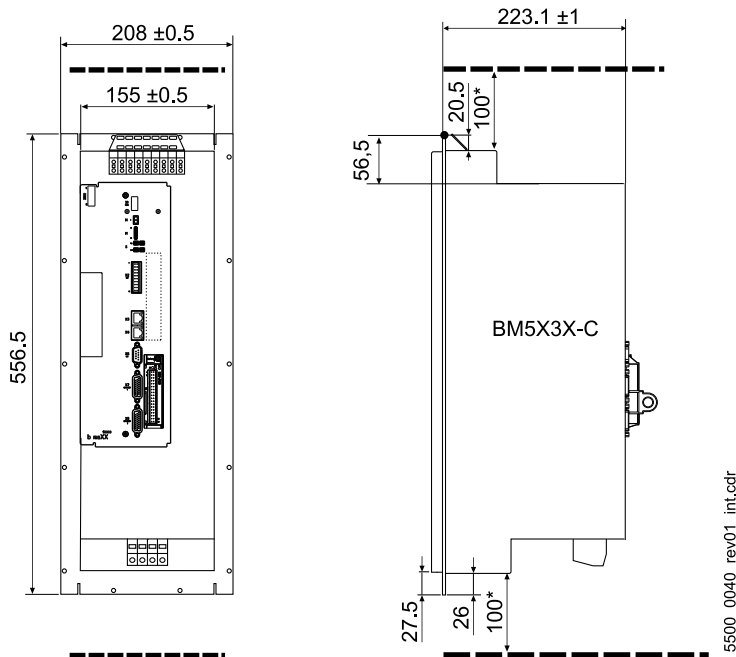
Figure 10: Dimensions BM553X-C
