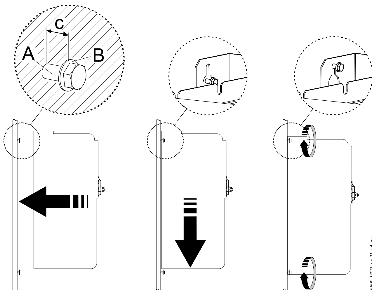
Abbildung 74: Mounting instruction BM555X-S/Z, BM556X-S/Z
