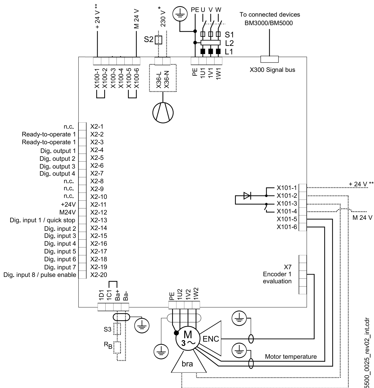
Abbildung 83: Connection diagram with a directly controlled motor brake - basic units
