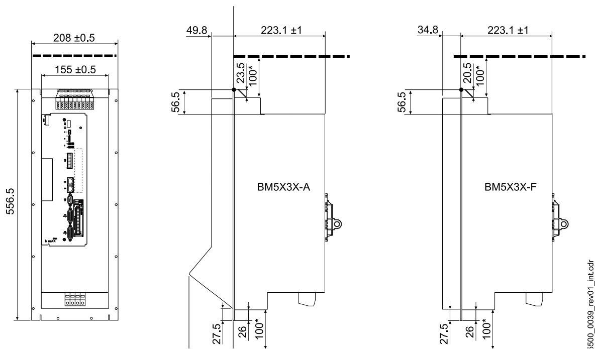
Figure 9: Dimensions BM553X-A/F
