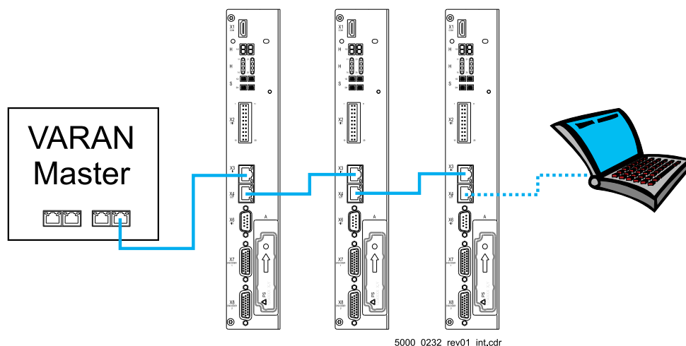
Figure 106: VARAN fieldbus connection
