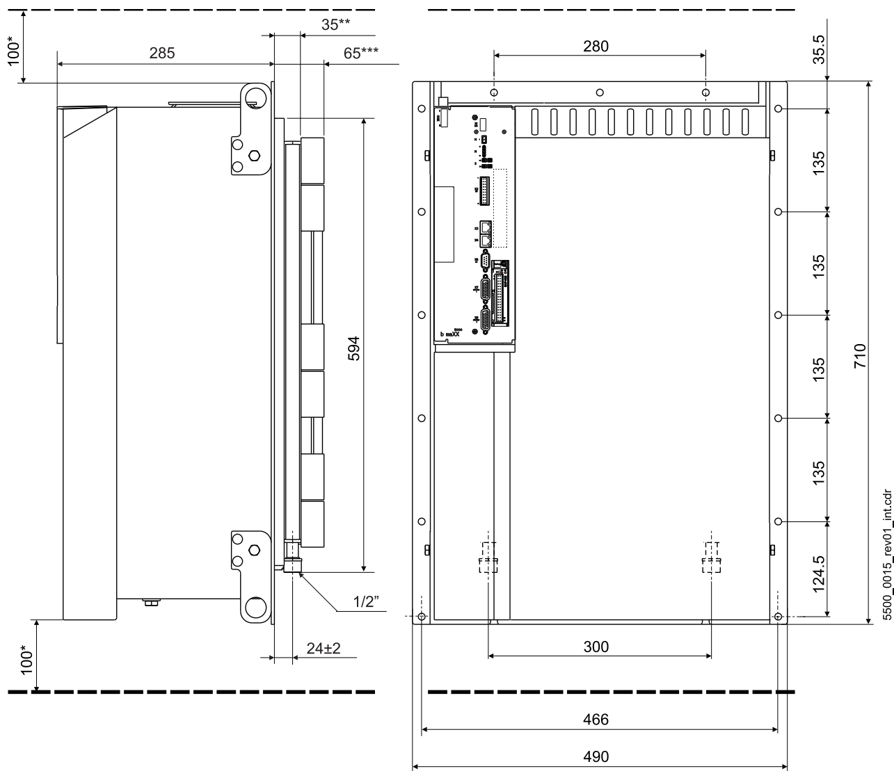
Figure 22: Dimensions BM566X-FXX9, BM576X-FXX9
