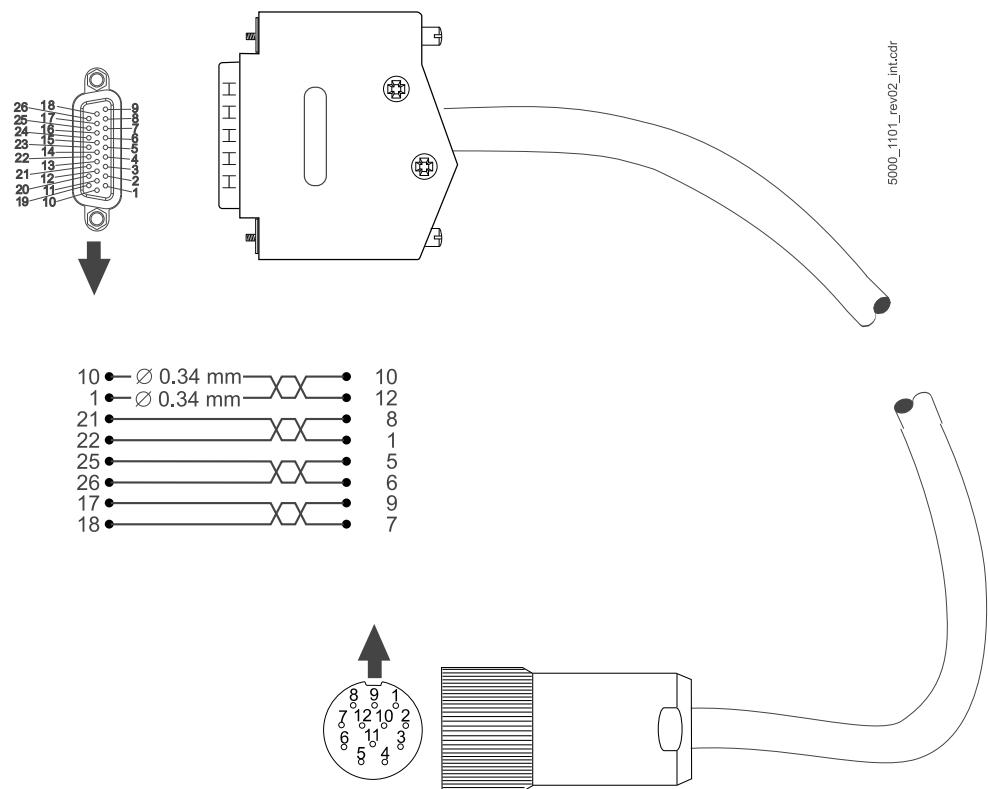
Figure 113: Connecting cable for resolver
