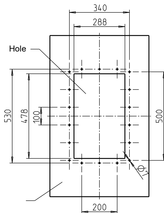
Figure 68: Drilling pattern BM565X-FXX9, BM575X-FXX9
