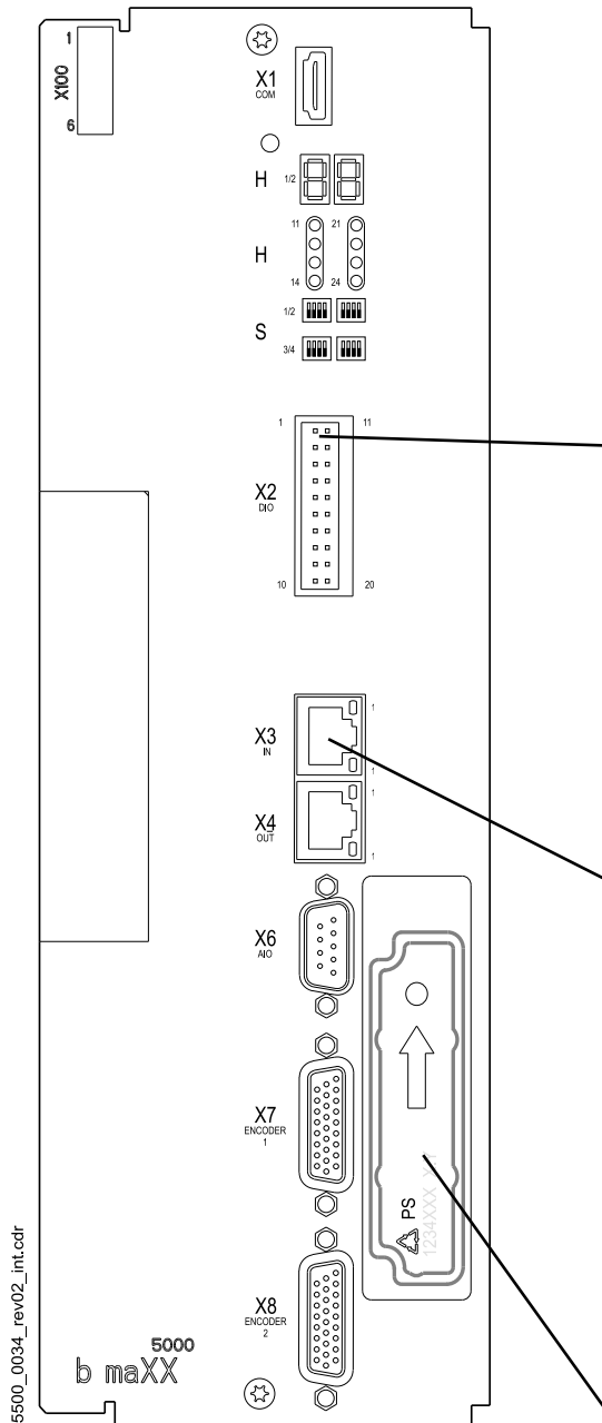
Figure 98: Connections controller
