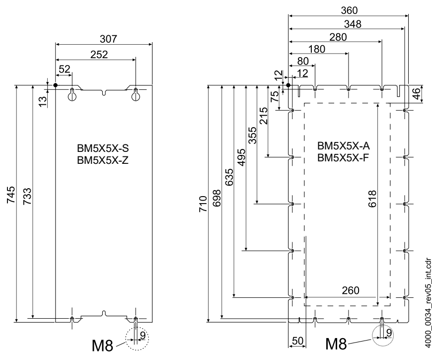
Figure 67: Drilling pattern BM555X, BM565X
