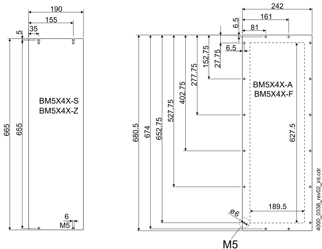
Figure 65: Drilling pattern BM554X, BM564X
