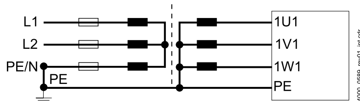
Figure 80: Connection to single phase grounded power supply systems with an isolated transformer
