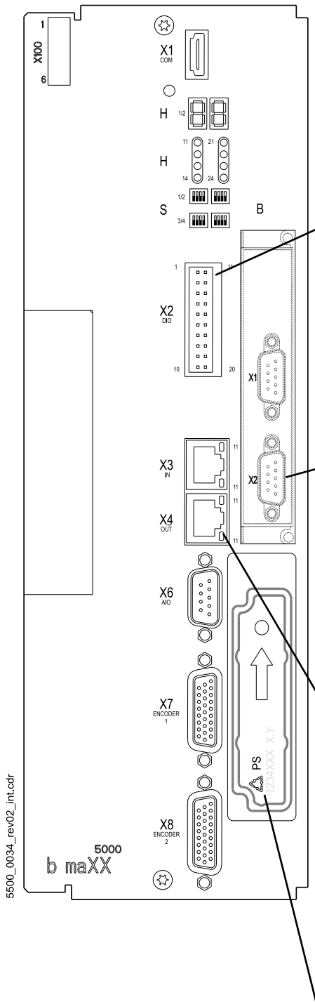
Figure 99: Connections controller
