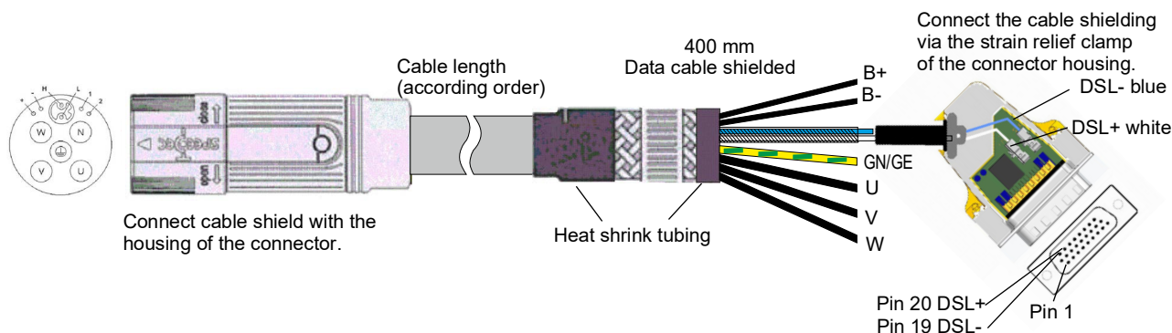
Figure 110: Motor cable with HIPERFACE DSL® 21 A
