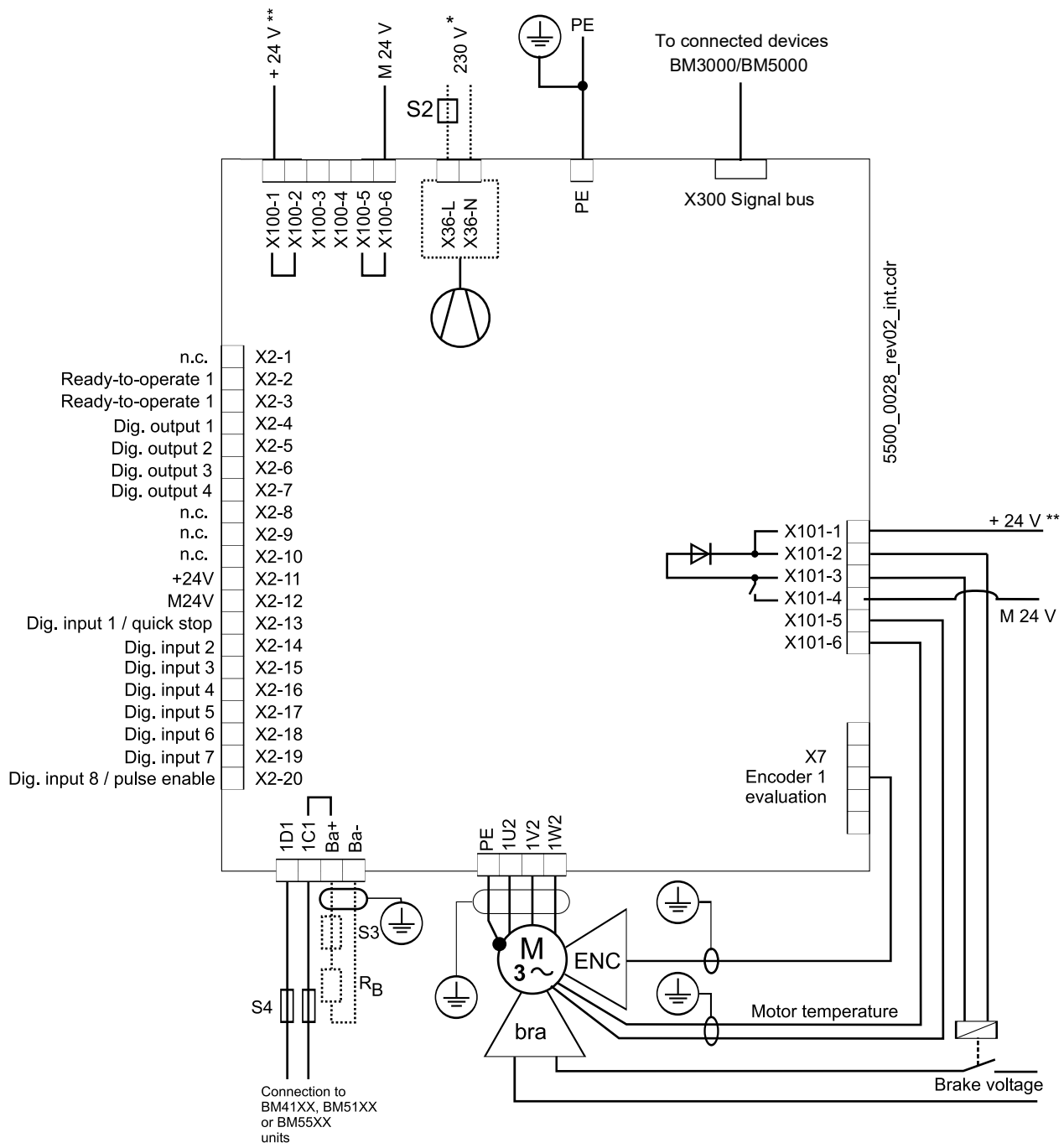
Abbildung 86: Connection diagram with motor brake controlled via an additional relay - power modules
