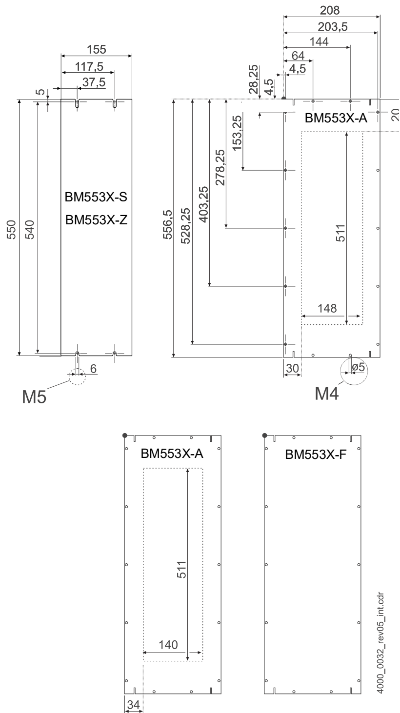
Figure 64: Drilling pattern BM553X, BM563X
