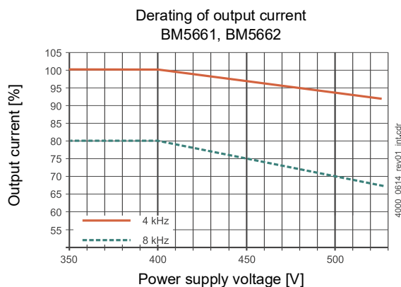
Figure 45: Derating the output current BM566X acceleration units
