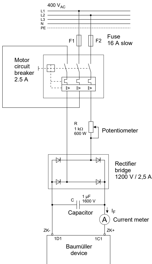
Figure 125: Connecting diagram forming
