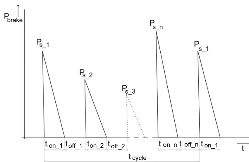
Figure 54: Braking cycle
