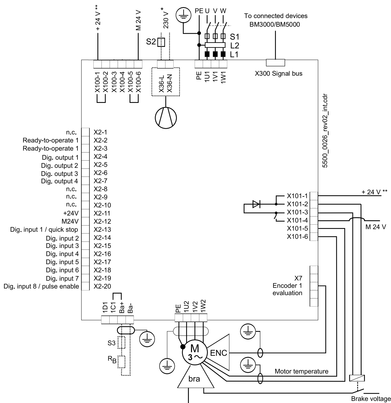
Abbildung 84: Connection diagram with motor brake controlled via an add. relay - basic units
