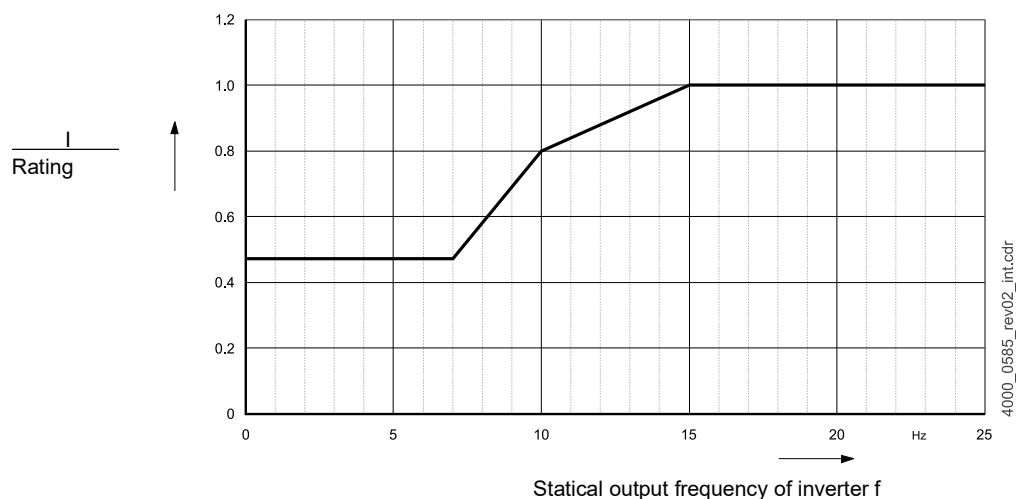
Figure 55: Derating at a static inverter frequency < 15 \text{ Hz}
