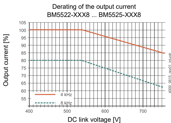
Figure 47: Derating the output current BM552X power modules
