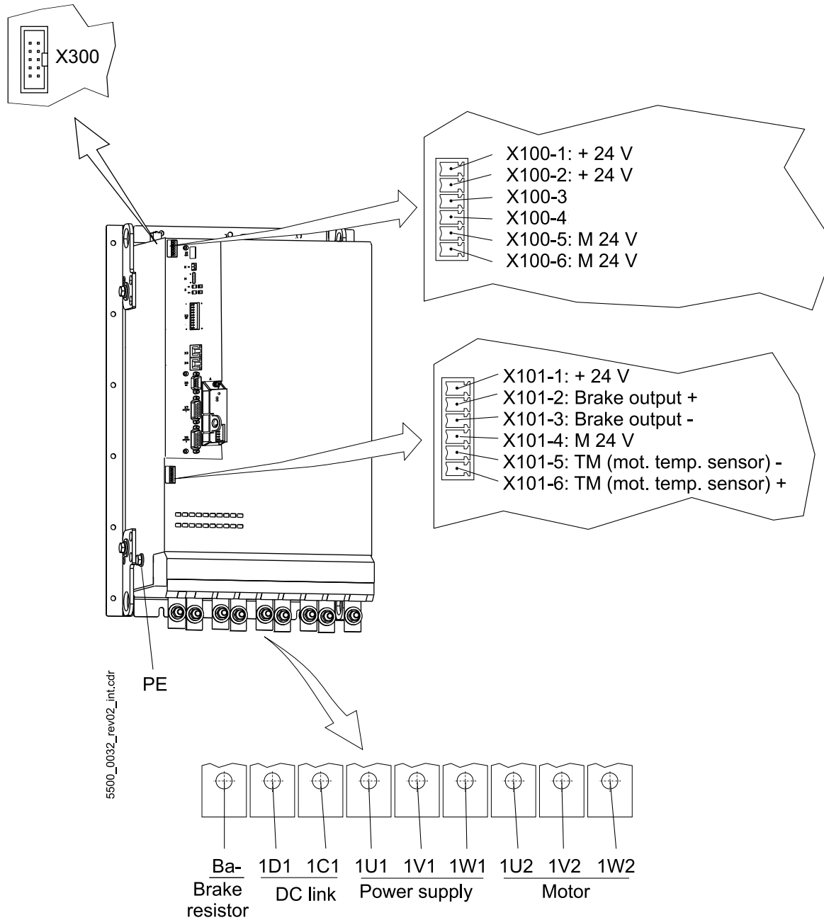
Figure 96: Electrical connections for power supply, motor, .. for BM5755
