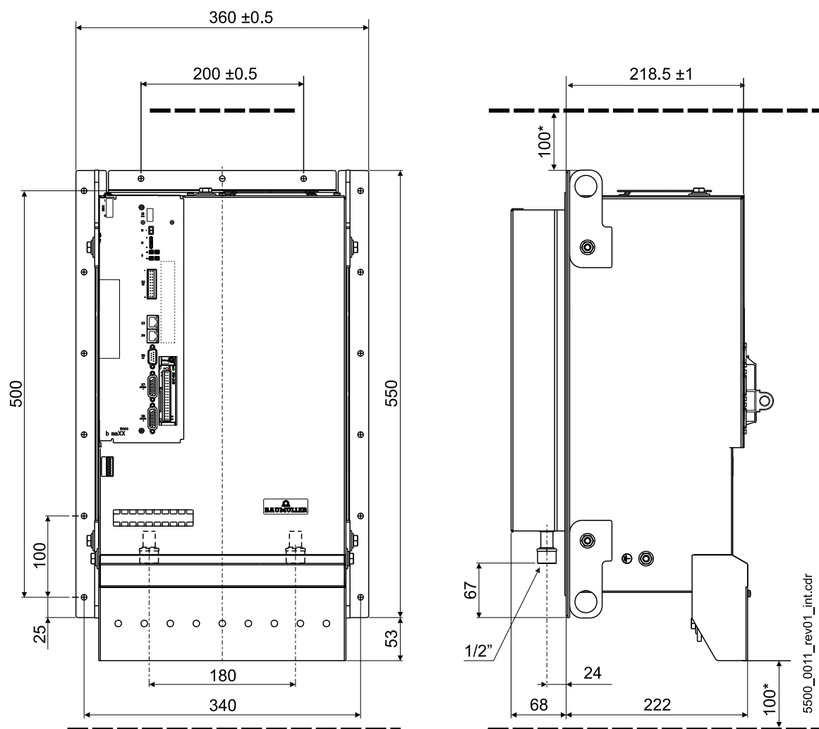
Figure 18: Dimensions BM575X-FXX9-RYY *: Observe minimum clearance, Observe ►Cooling◄ from page 58.
